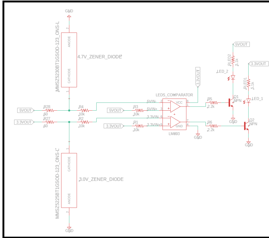
Figure 6.4. Schematic Capture of the Voltage Regulator Status LED Circuit
