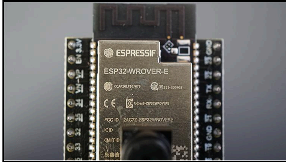
Figure 3.5. PCB Trace Antenna on ESP32-WROVER-E
