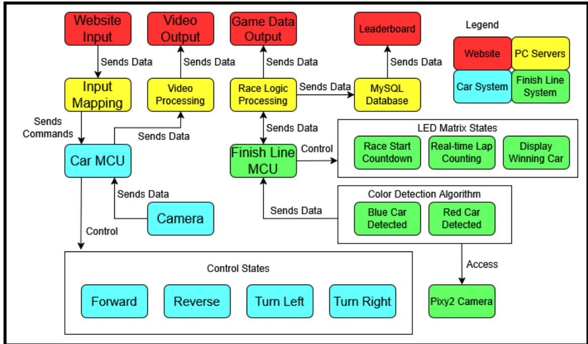
Figure 7.2. Functionality Block Diagram
