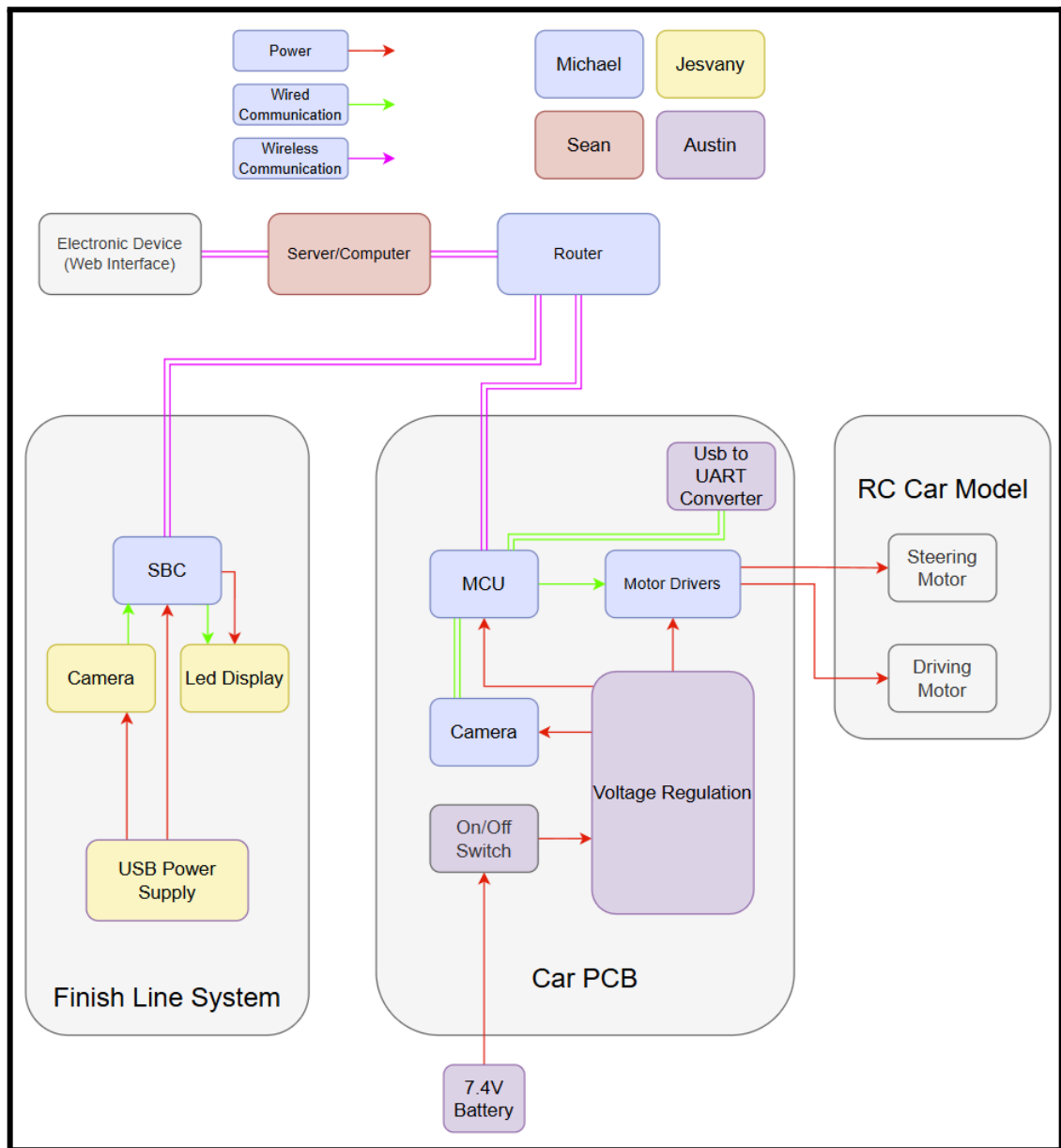
Figure 2.1. Hardware Block Diagram
