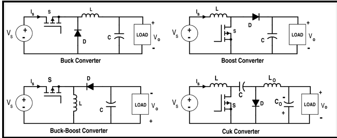
Figure 3.9. Basic Converters Design (Analysis of DC-DC Converters in Equilibrium, All About Circuits technical article)
