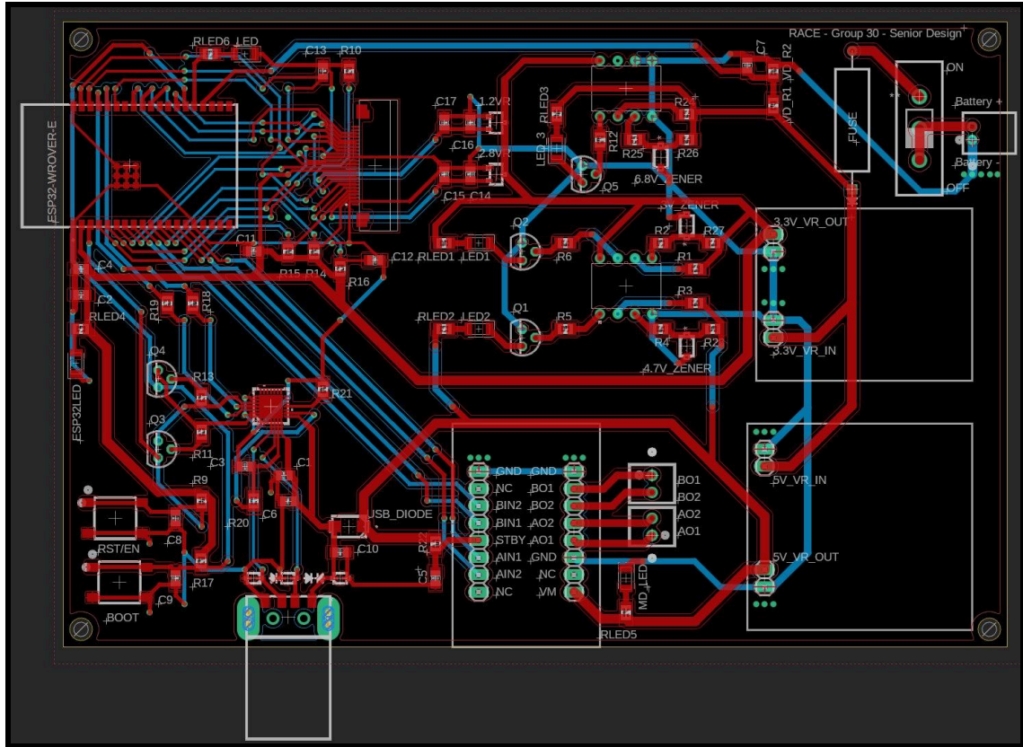
Figure 8.4. Complete PCB Design
