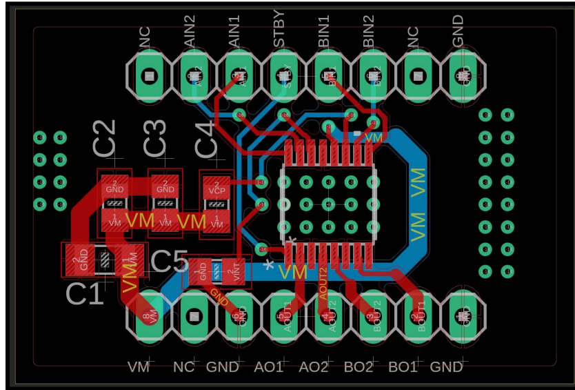
Figure 8.3. Motor Driver PCB Design
