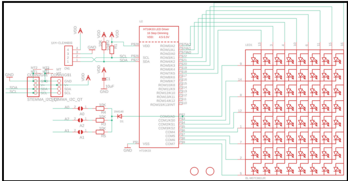
Figure 6.16. Schematic Capture of Bi-Color LED Matrix with I2C Backpack
