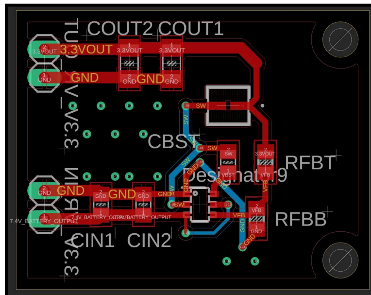
Figure 8.2. 3.3 V Regulator PCB Design
