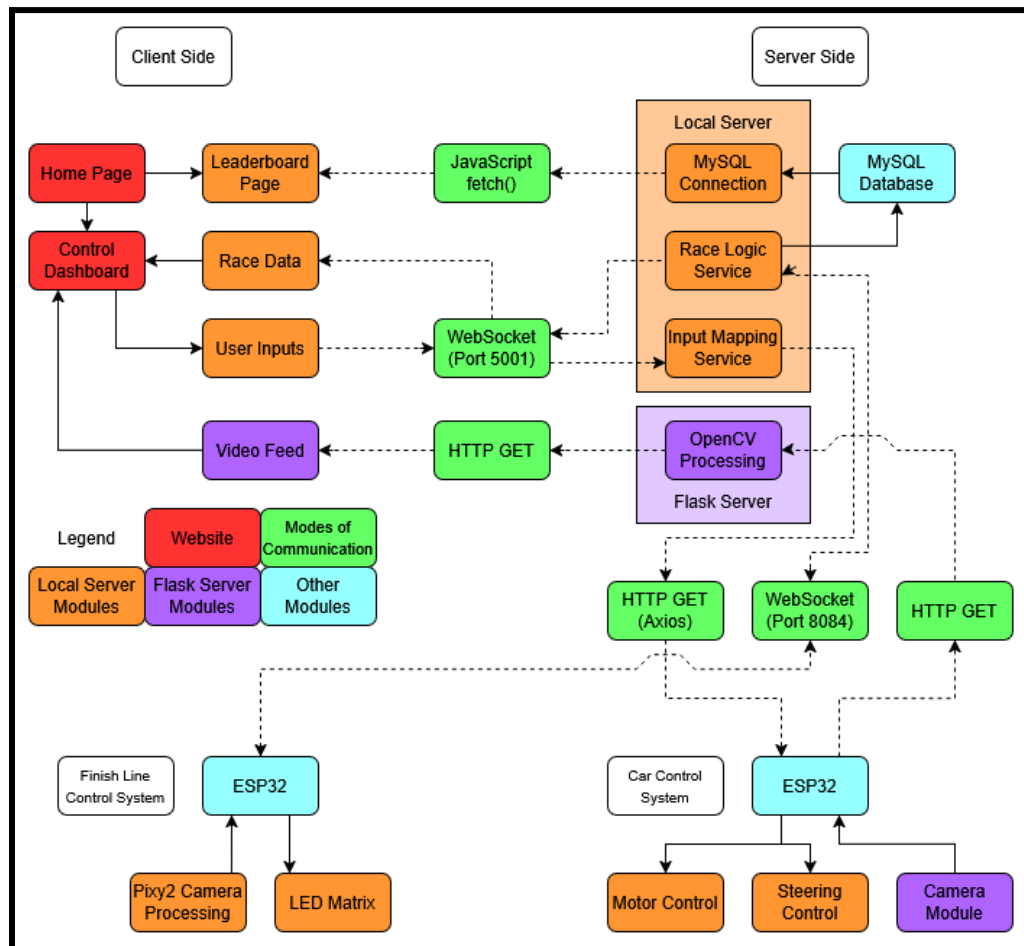
Figure 7.1. Signals Block Diagram
