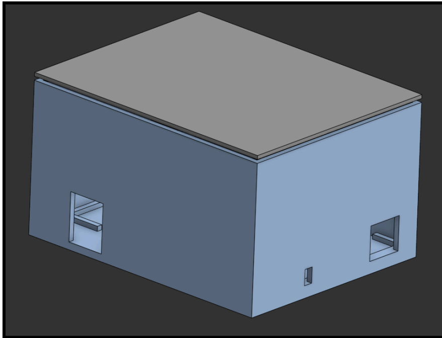
Figure 8.6. 3D Model of IC Car PCB Enclosure
