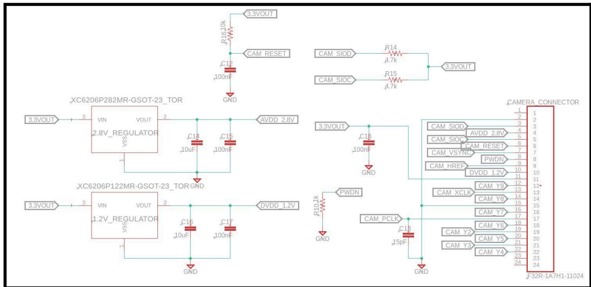
Figure 6.8. Schematic Capture of OV2640's Camera Connector
