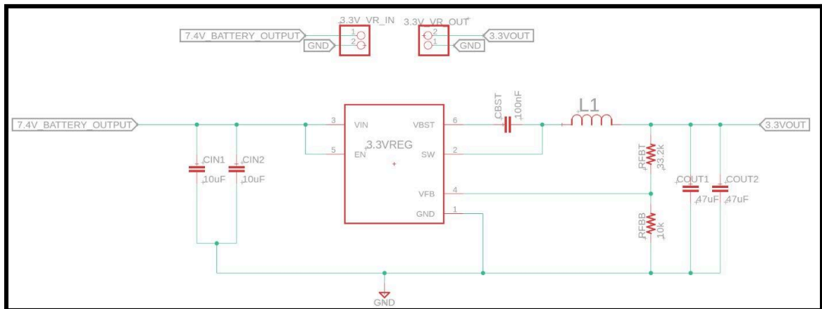
Figure 6.2. Schematic for the 3.3 V Regulator Circuit
