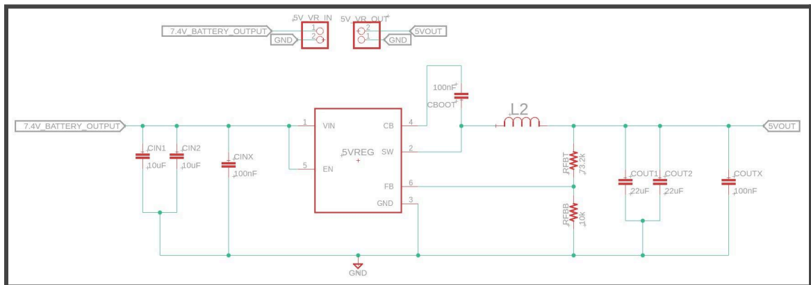
Figure 6.3. Schematic for the 5 V Regulator Circuit
