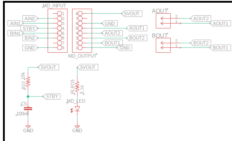
Figure 6.6. Schematic Capture of Motor Driver and Terminal Connections
