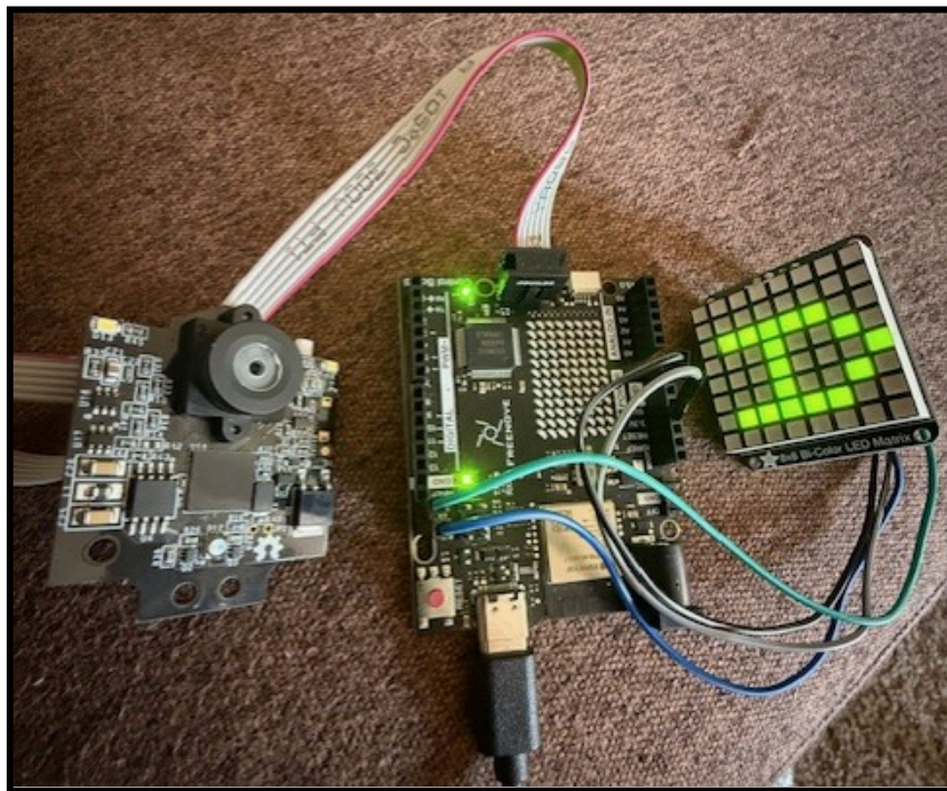
Figure 9.8. Photo of Pixy2, Freenove Control Board, and LED Matrix Integration
