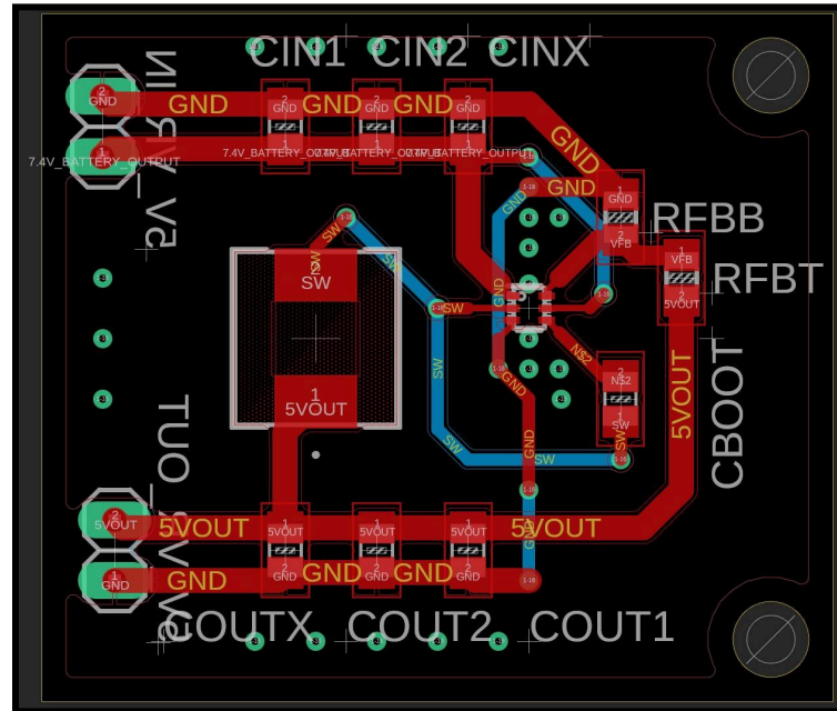
Figure 8.1. 5 V Regulator PCB Design
