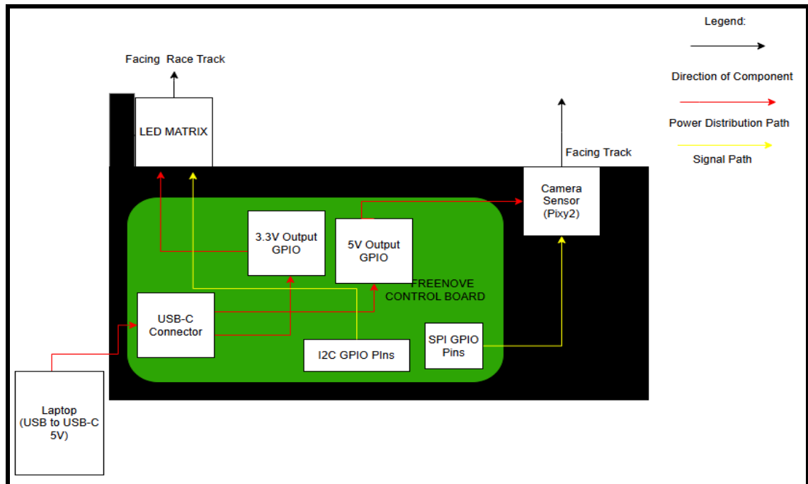
Figure 8.8. Block Diagram of Finish Line Enclosure
