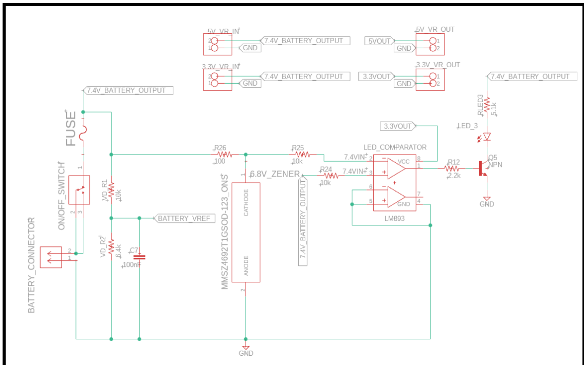
Figure 6.5. Schematic Capture of Battery Voltage Monitor and Terminal Connection
