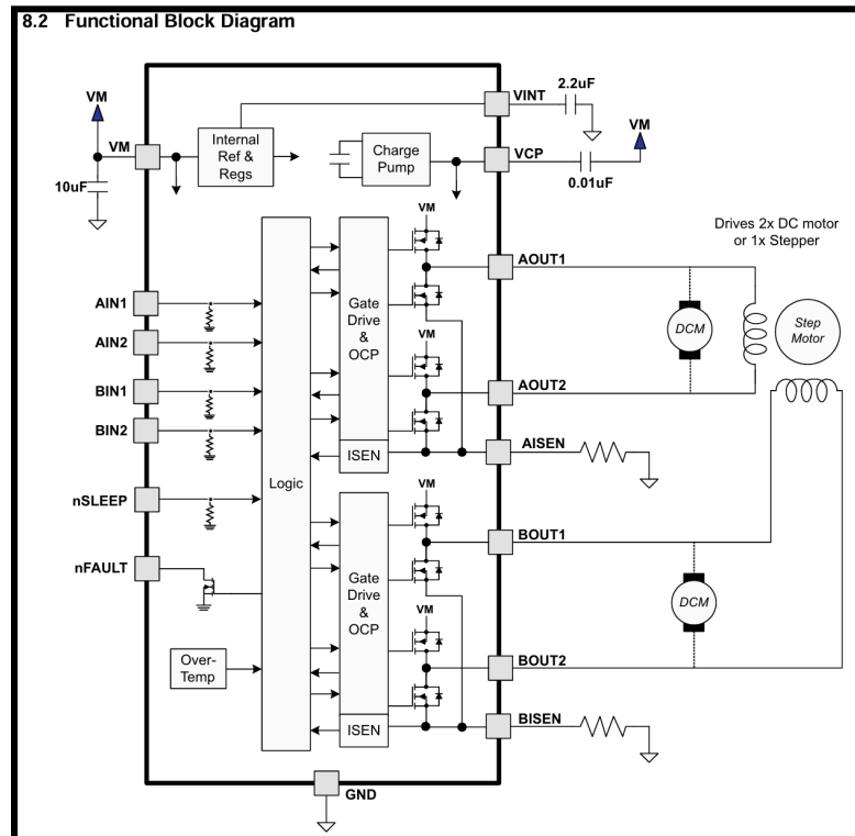
Figure 6.7. DRV8833 Functional Block Diagram via TI Datasheet
