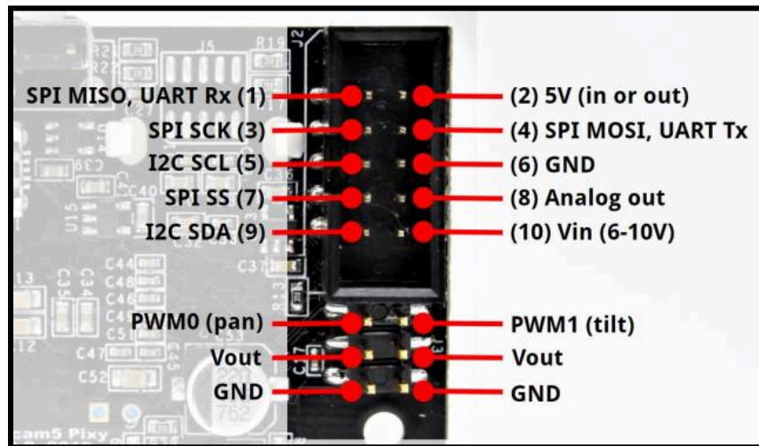
Figure 6.15. Pixy2 Camera Pinouts
