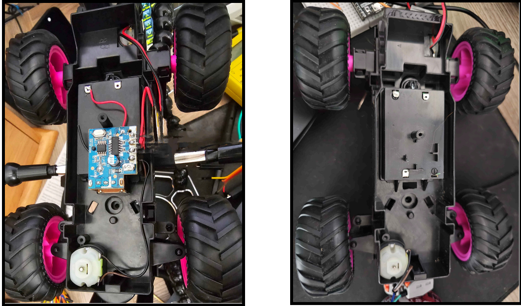
Figure 6.13. RC Car Original Setup (Left) and Removal of Parts (Right)
