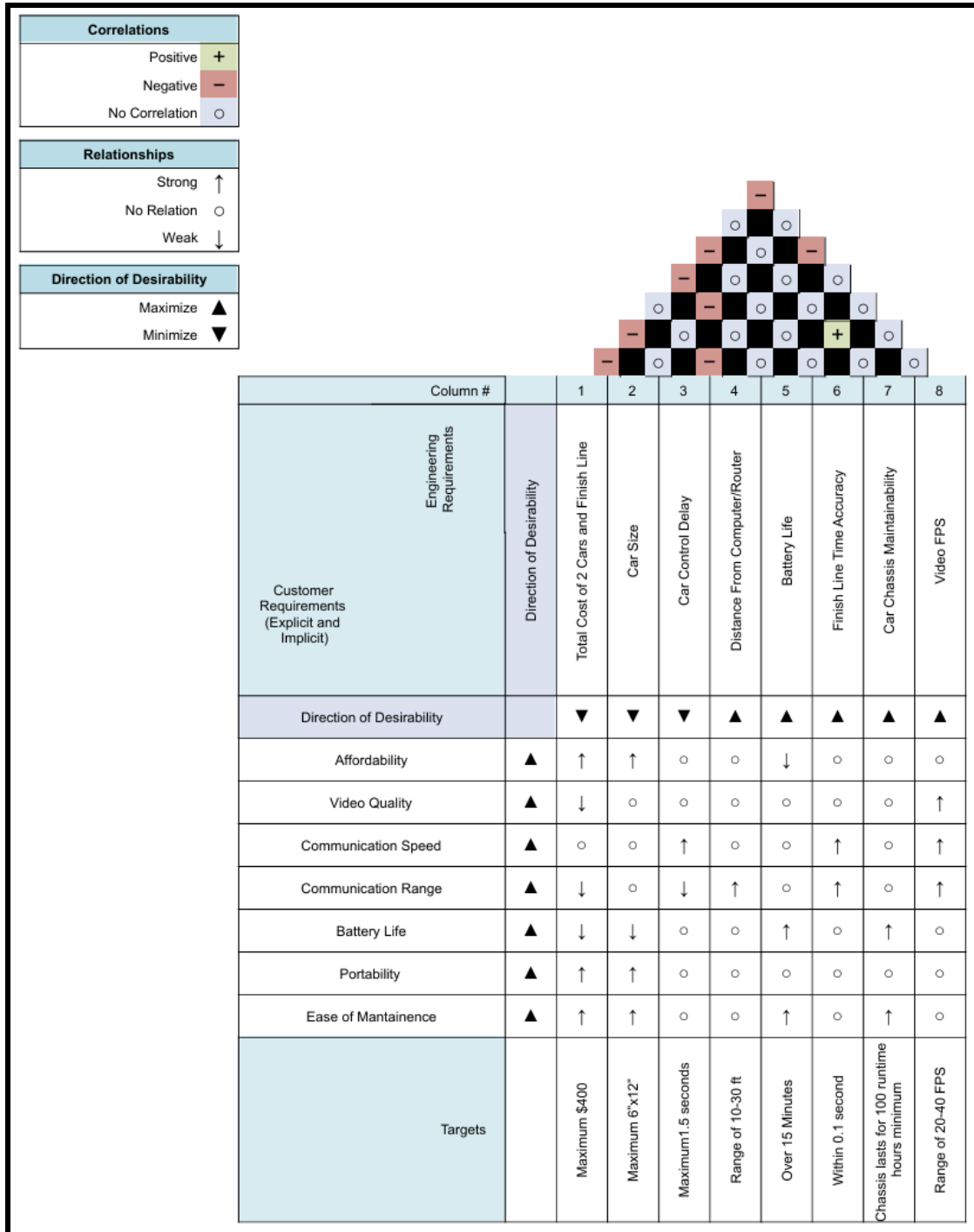
Figure 2.3. House of Quality Table
