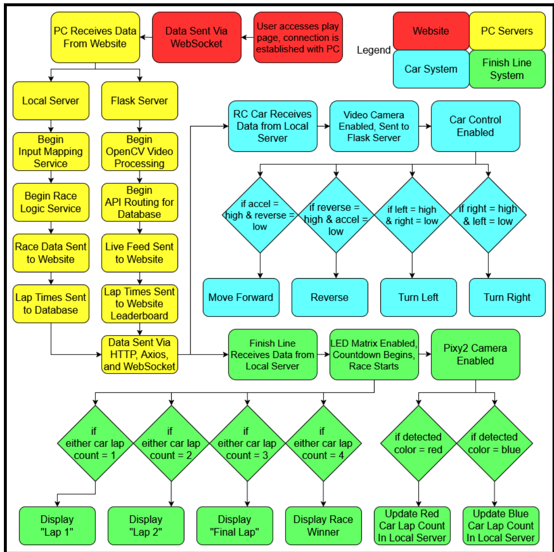
Figure 2.2. Software Flowchart
