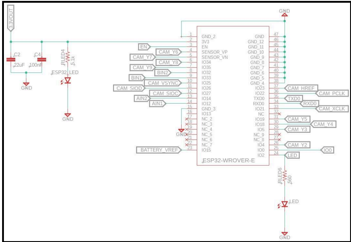
Figure 6.10. Schematic Capture of ESP32 Connections
