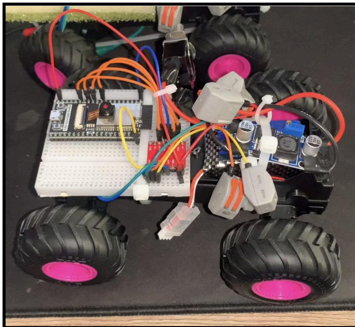
Figure 6.14. IC Car Breadboard Prototype
