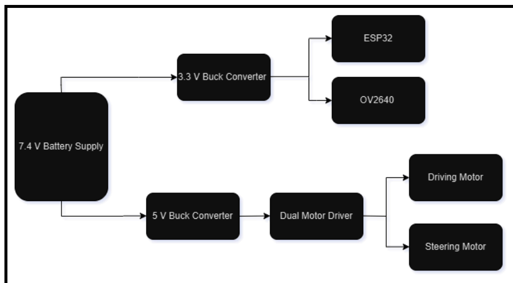
Figure 6.1. Cars System Power Supply Architecture
