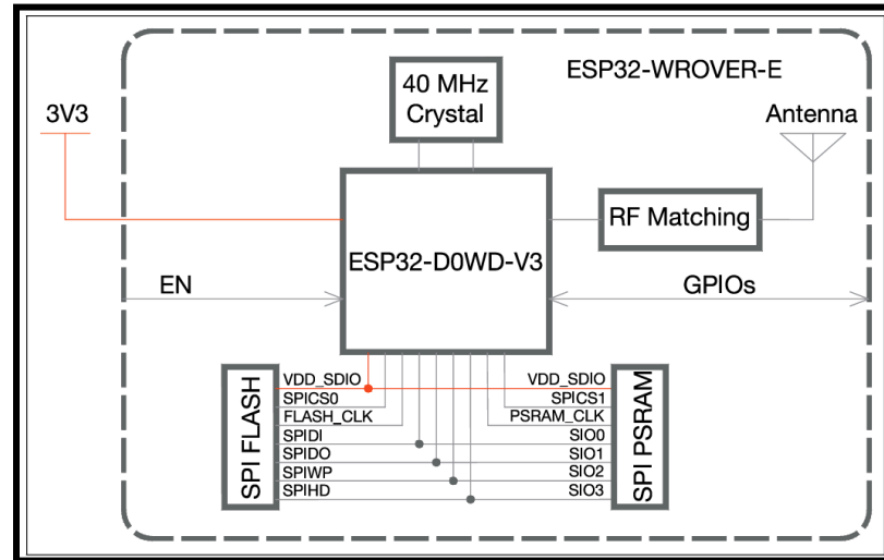
Figure 6.12. ESP32-WROVER-E Module Block Diagram
