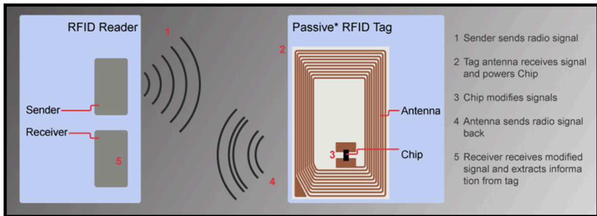
Figure 3.4. Passive RFID Example
